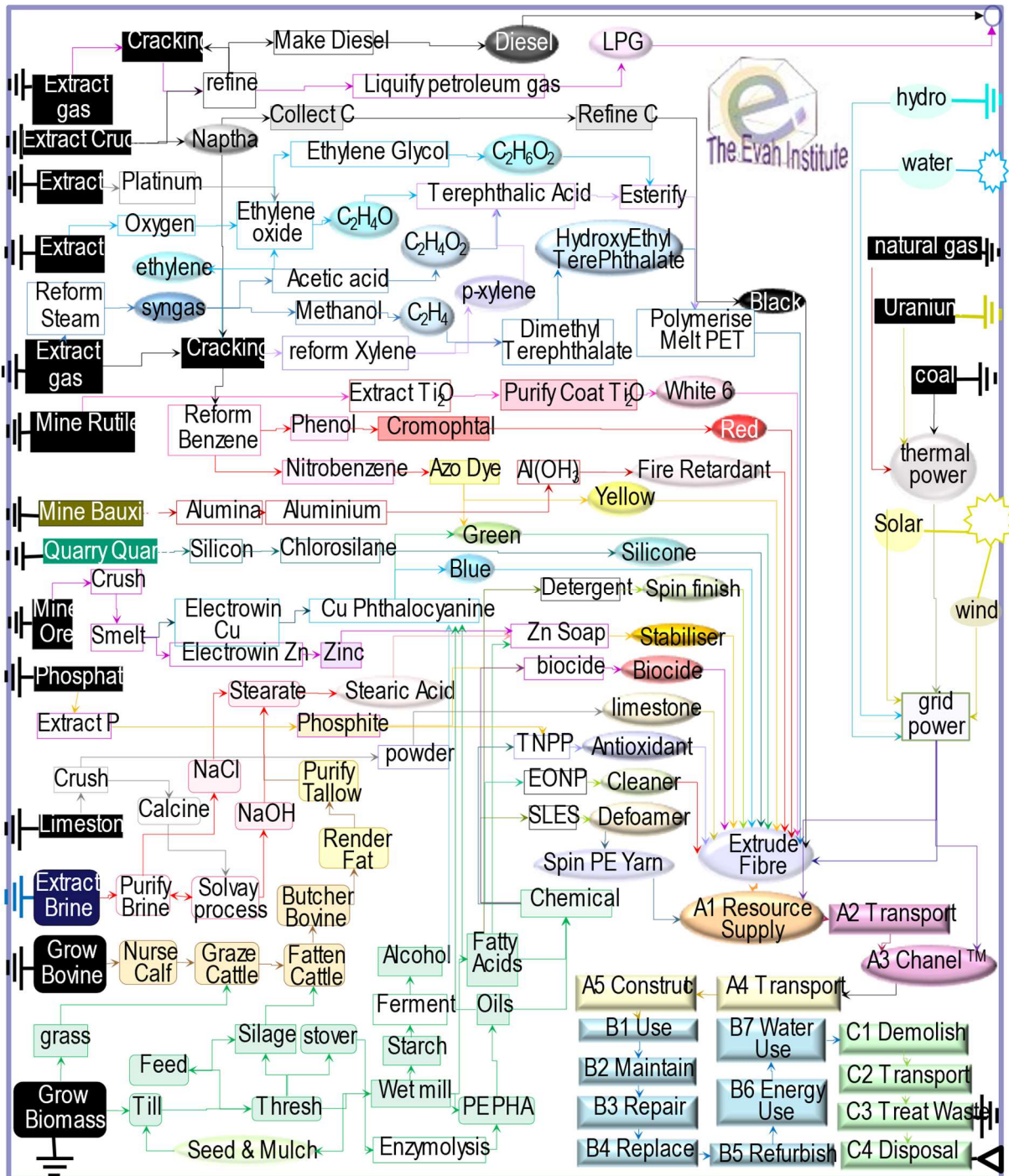
Figure 2. Product Process Flow Chart Completeness
