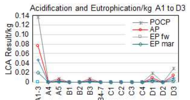
Figure 6 POCP, AP & EP/kg A1 to C4
