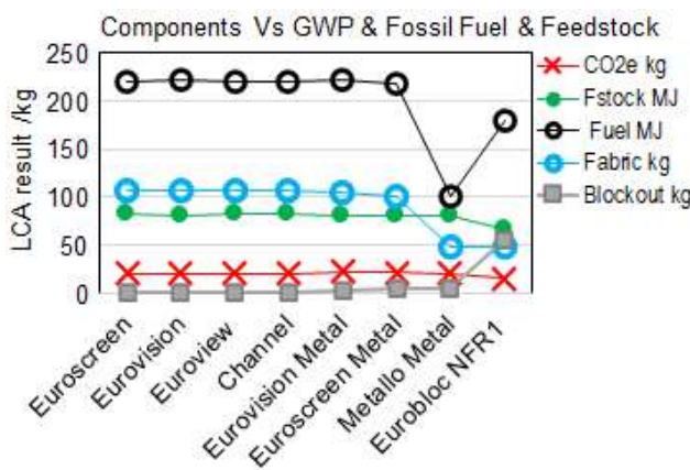
Figure 3 A1-A3 Component & EE% share//kg
