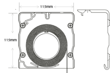
115mm HEADBOX
